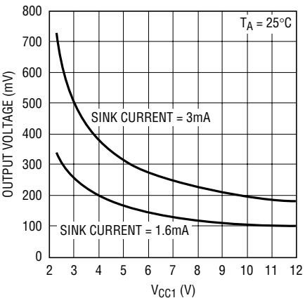
RESET, FAULT, COMPOUT Output Voltage vs V CC1
