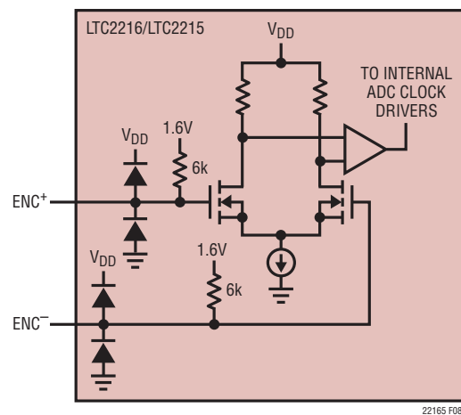
Figure 8. Equivalent Encode Input Circuit
