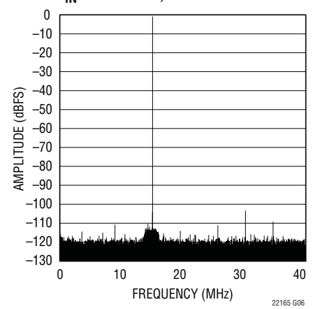
LTC2216 64k Point FFT, f_{IN} = 15.1\text{MHz} , -1dBFS
