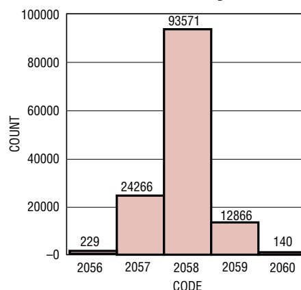
LTC2220: Noise Histogram
