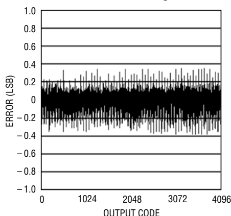
LTC2220: DNL, 2V Range
