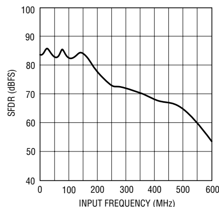
LTC2220: SFDR (HD2 and HD3) vs Input Frequency, -1dB, 2V Range, LVDS Mode
