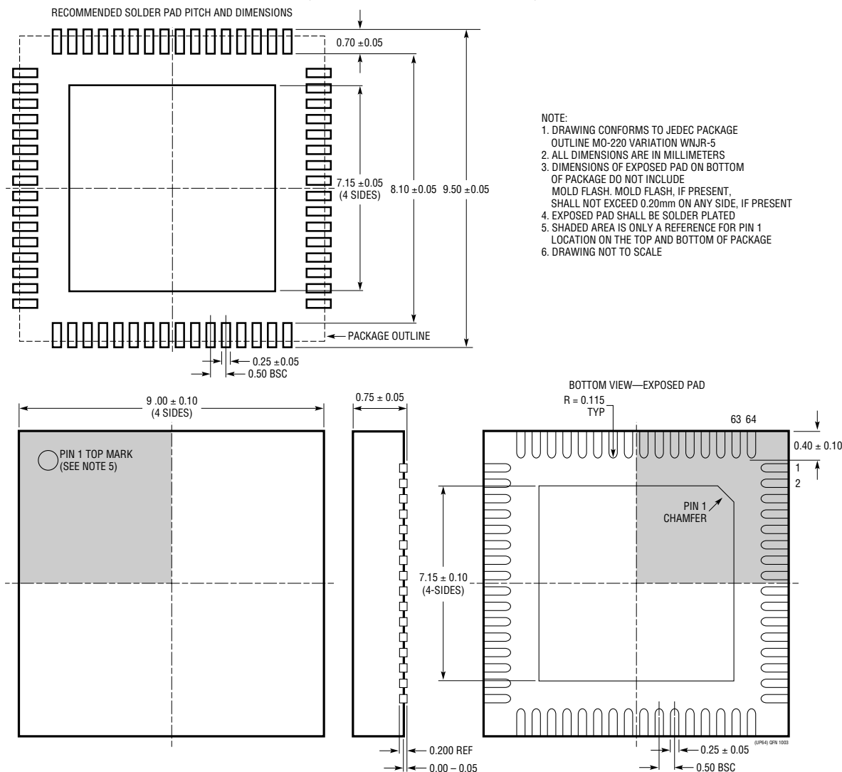
UP Package 64-Lead Plastic QFN (9mm × 9mm) (Reference LTC DWG # 05-08-1705)
