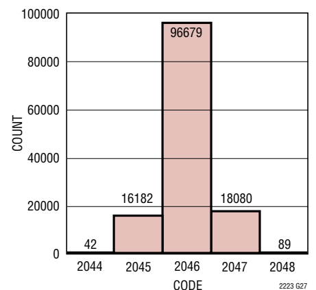
LTC2223: Noise Histogram
