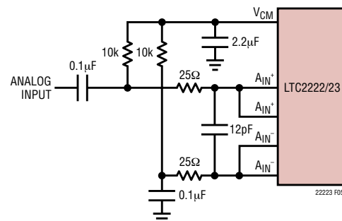
Figure 5. Single-Ended Drive
