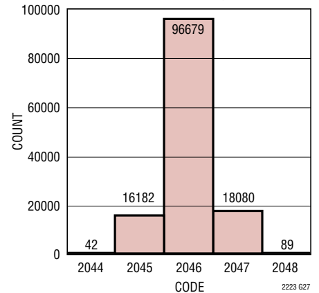
LTC2222: Noise Histogram
