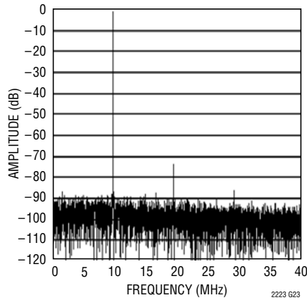
LTC2222: 8192 Point FFT, f_{IN} = 250\text{MHz} , -1\text{dB} , 1V Range
