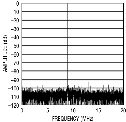
LTC2227: 8192 Point FFT, f_{IN} = 30\text{MHz} , -1dB, 2V Range, 40Msps
