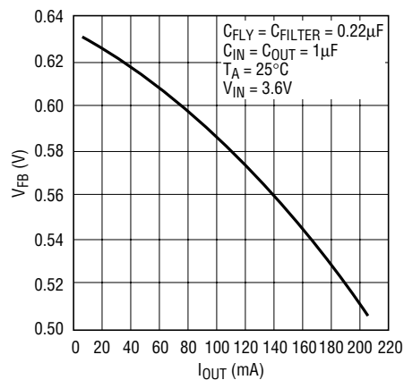
Feedback Voltage vs I_{OUT}
