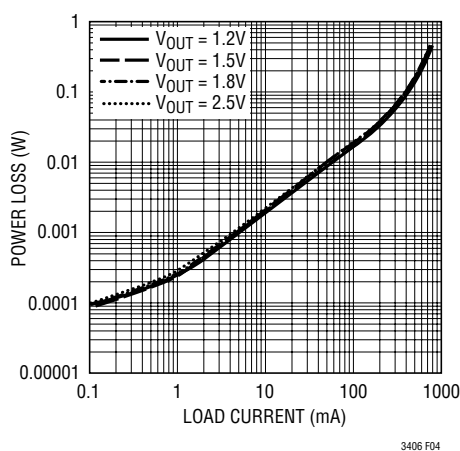
Figure 4. Power Lost vs Load Current
