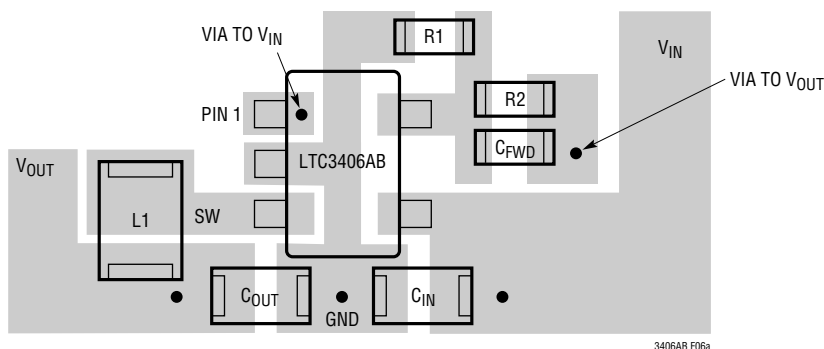
Figure 4. LTC3406AB Suggested Layout
