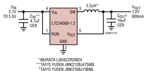
Figure 1. Typical Application
