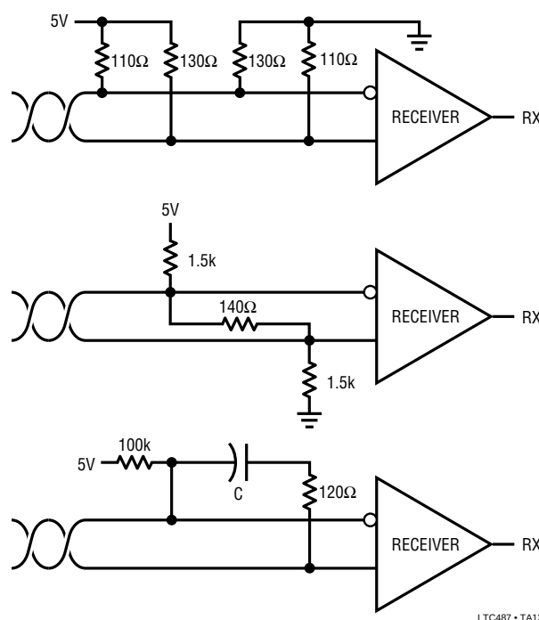
Figure 11. Forcing '0' When All Drivers Are Off
