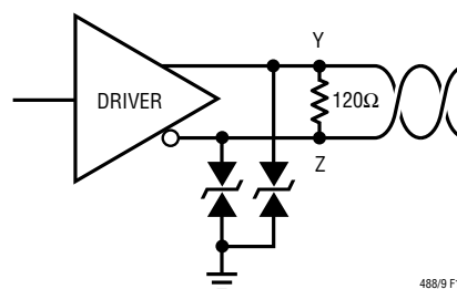
Figure 11. ESD Protection with TransZorbs®
