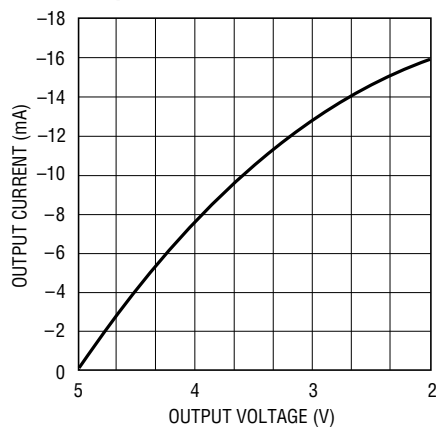
Receiver Output High Voltage vs Output Current at T_A = 25^\circ\text{C}
