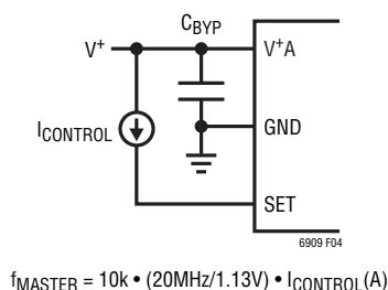
Figure 4. Current Controlled Oscillator
