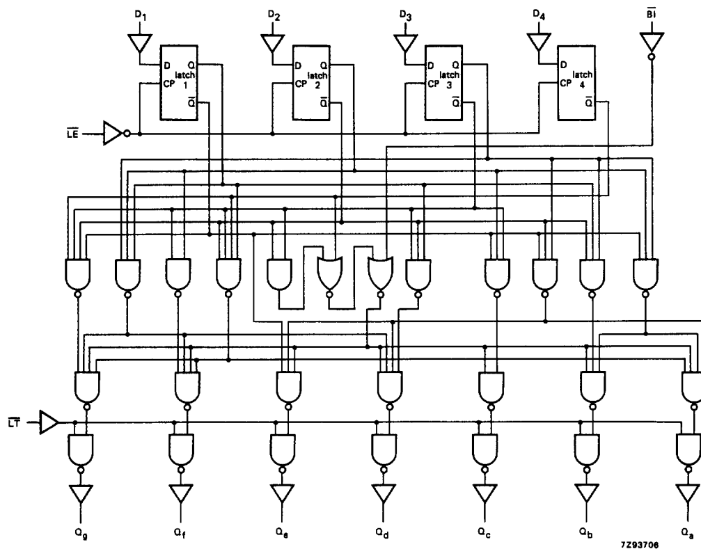
Fig.5 Logic diagram.
