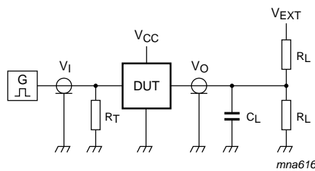
Test data is given in Table 10 . Definitions for test circuit: R_L = Load resistance. C_L = Load capacitance including jig and probe capacitance. R_T = Termination resistance; should be equal to the output impedance Z_o of the pulse generator. V_{EXT} = External voltage for measuring switching times.
