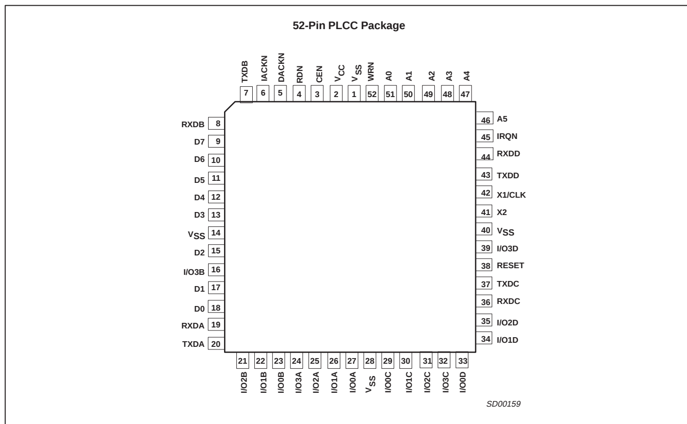
Figure 1. Pin configuration
