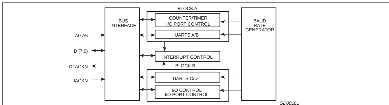
Figure 3. Channel Architecture
