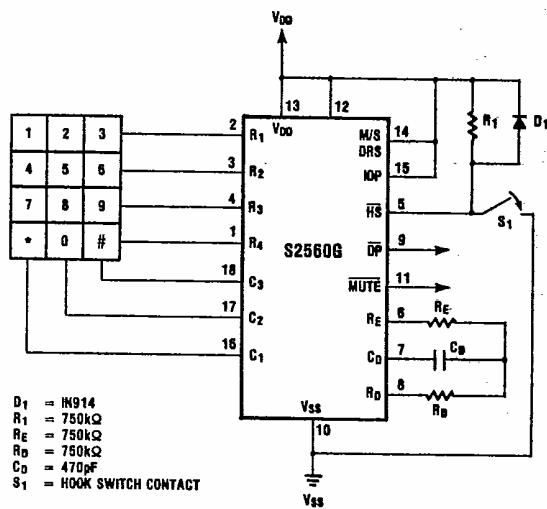
Figure 1. Transient Protection Technique Using Diode Between V_{DD} and HS
