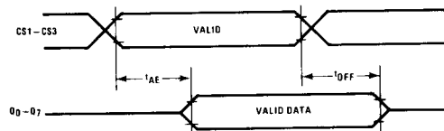
Propagation Delay From Chip Enable
