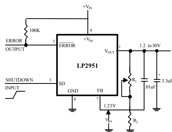
Figure 1. Adjustable Regulator
