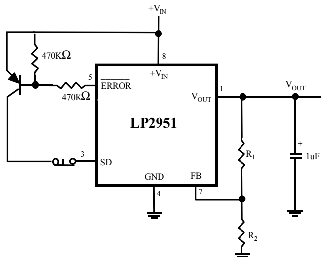
Fig.2 Latch Off When Error Flag Occurs
