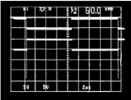
Receiver Output
