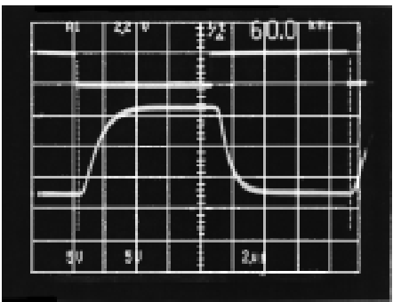
Transmitter Output R L =3kΩ, C L =2,500pF
