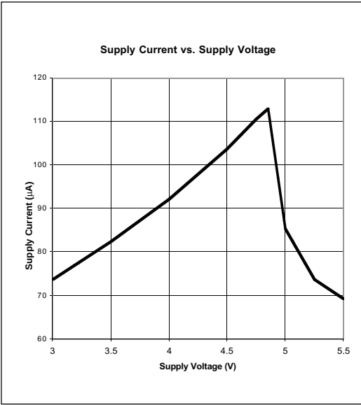
Figure 10. On-state Supply Current vs. Supply Voltage
