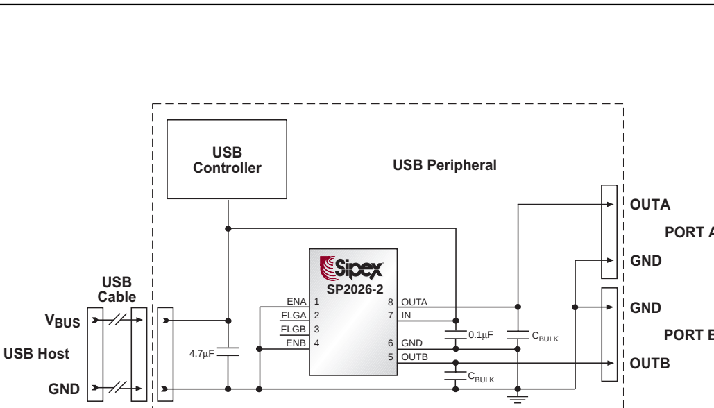
Figure 5. Soft Start Circuit Configuration for a Single Channel USB-powered Application with the SP2026
