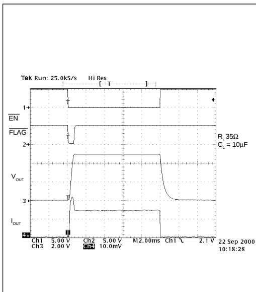
Figure 19. Turn-on/Turn-off Characteristics Where R_L = 35\Omega and C_L = 10\mu F
