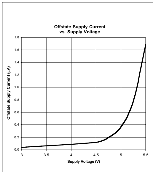
Figure 13. Off-state Supply Current vs. Supply Voltage
