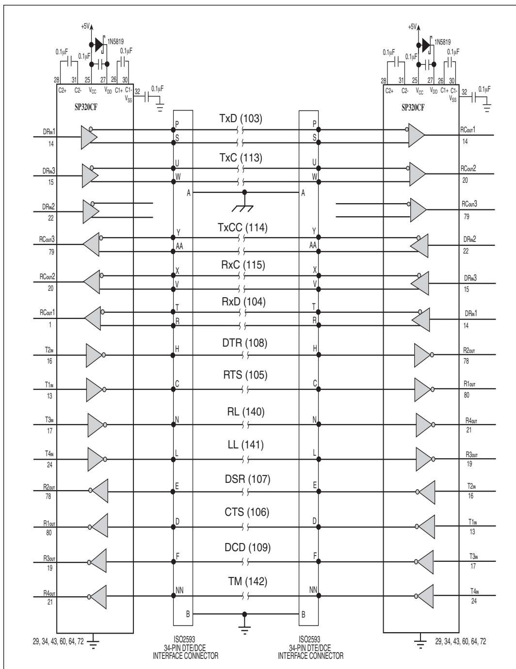
Figure 7. Typical DTE-DCE V.35 Connection with the SP320
