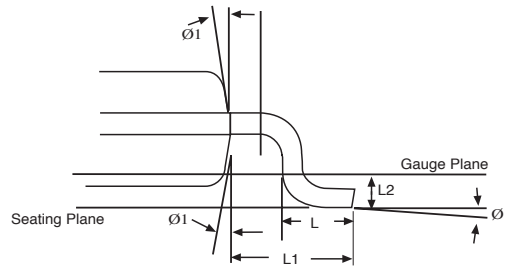
VIEW C
