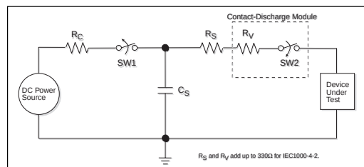
Figure 7. ESD Test Circuit for IEC1000-4-2
