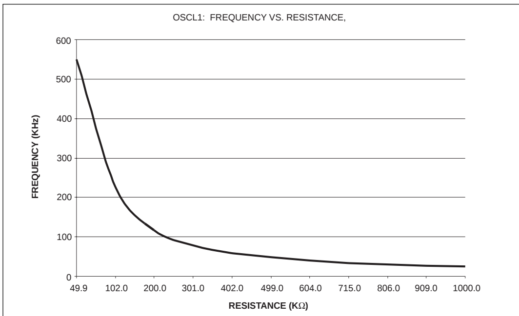
Figure 7. Oscillator Frequency vs R_{OSC} , V_{DD}=3.0V
