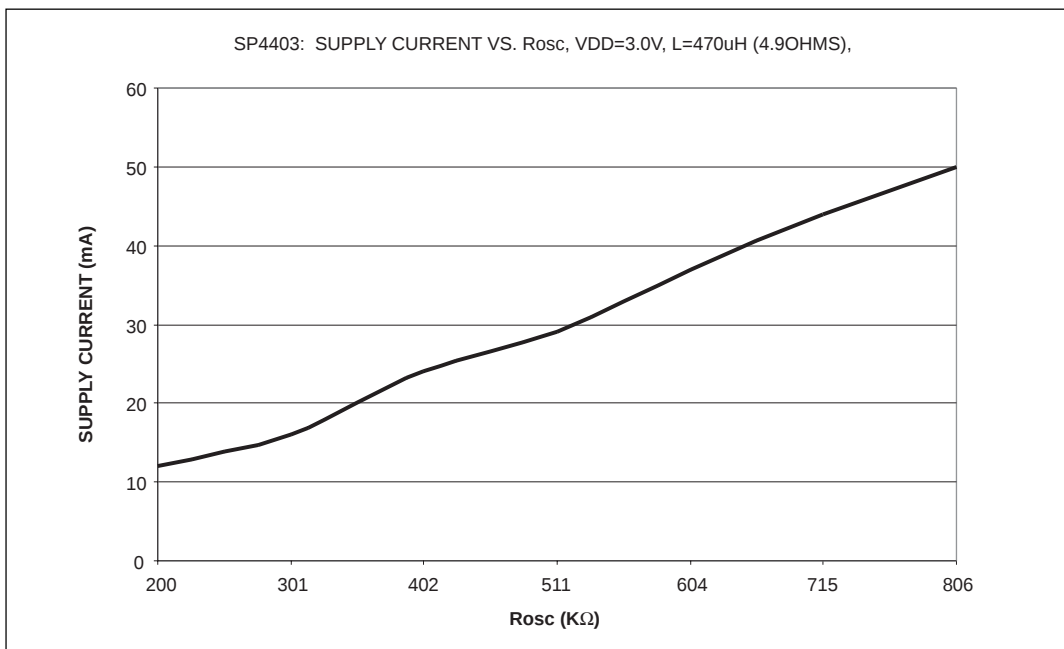
Figure 8. I_{TOTAL} vs R_{OSC} , V_{DD}=3.0V , Coil=470 \mu H , 4.9 \Omega
