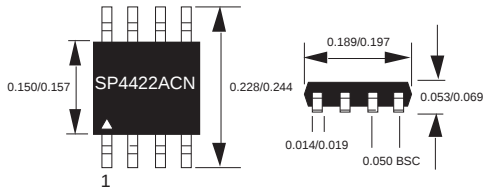
8-pin NSOIC
