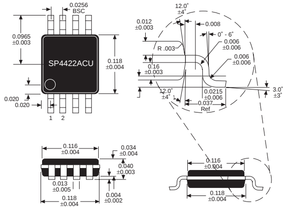
8-pin \mu SOIC
