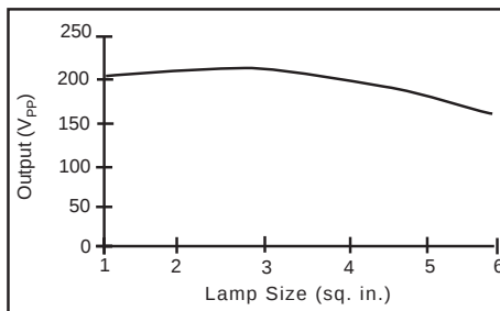
Output Voltage vs. Lamp Size. V_{DD} = 3.0V ; Coil= 5mH, 18 \Omega ; C_{OSC} = 100pF
