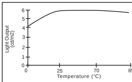
Light Output vs. Temperature V_{DD}=3.0V ; Coil=5mH/18Ω; C_{OSC}=100pF ; Lamp=6sq.in.
