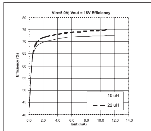
Figure 6. 18V Output Efficiency ( V_{IN}=5\text{V} )
