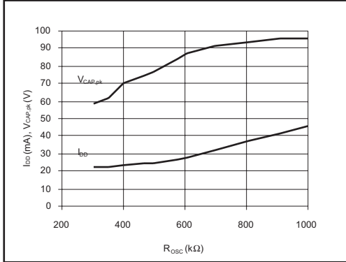
Figure 3: Supply Current and Cap Pin Voltage vs. Oscillator Resistance.
