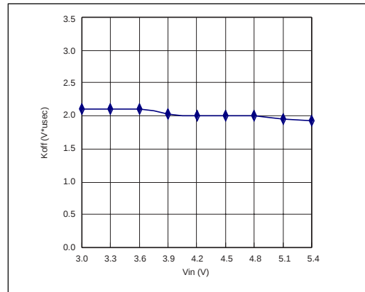
K_{OFF} vs V_{IN} , V_{OUT} = 1.5\text{V}
