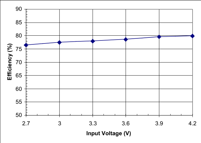
Fig. 1 Efficiency vs Input Voltage
