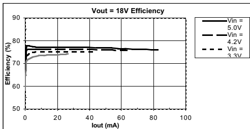
Figure 5. 18V Output Efficiency
