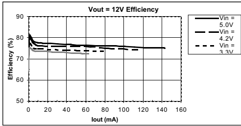
Figure 1. 12V Output Efficiency
