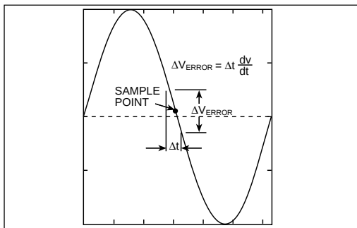
Figure 1. Aperture Uncertainty
