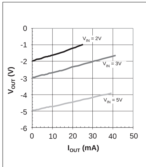
Figure 8. Output Voltage vs. Output Current with 0.1μF Capacitors
