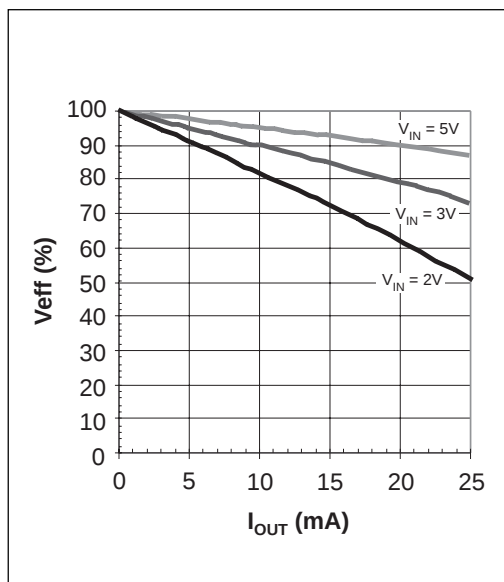
Figure 10. Voltage Efficiency vs. Output Current with 0.1μF Capacitors
