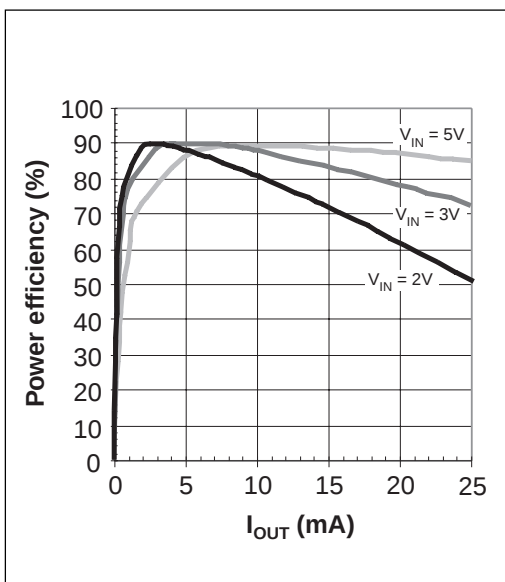
Figure 9. Power Efficiency vs. Output Current with 0.1μF Capacitors
