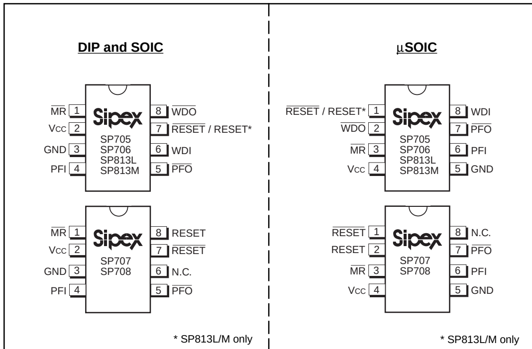
Figure 1. Pinouts
