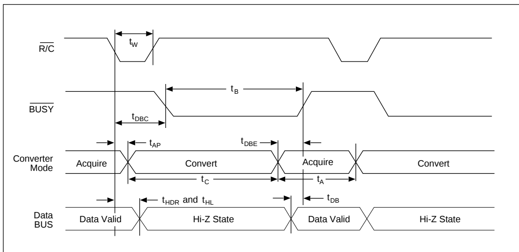
Figure 5. Convert Mode Timing — R/\overline{C} Pulse LOW, Outputs Enabled After Conversion
