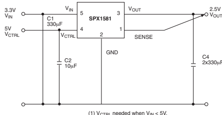
Typical Fixed Regulator
