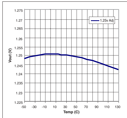
Figure 2. V_{OUT} vs Temperature, V_{IN}=2.5V , I_{OUT}=10mA
