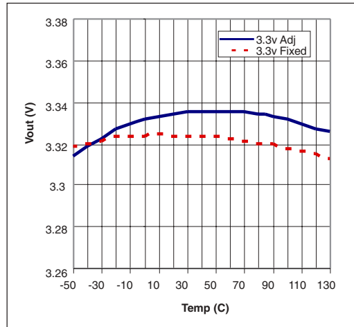
Figure 4. V_{IN}=5.0V , I_{OUT}=10mA
