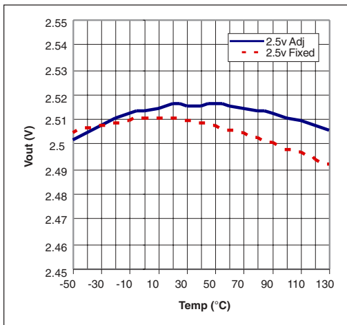
Figure 3. V_{IN}=4.0V , I_{OUT}=10mA
