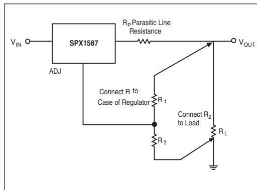
Figure 10. Recommended Connections for Best Results
