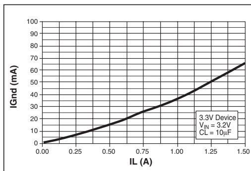
Figure 6. Ground Current vs Current in Dropout
