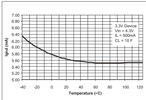
Figure 11. Ground Current vs Temperature at I_{LOAD}=500
