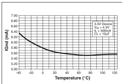
Figure 10. Ground Current vs Temperature at I_{LOAD} = 500\text{mA}
