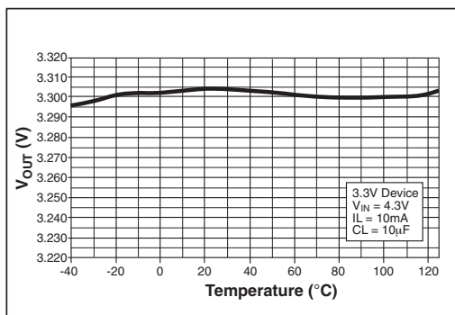
Figure 9. Output Voltage vs Temperature at I_{LOAD} = 10\text{mA}
