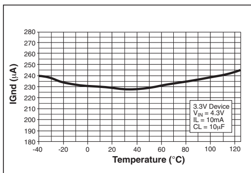
Figure 8. Ground Current vs Temperature at I_{LOAD} = 10\text{mA}
