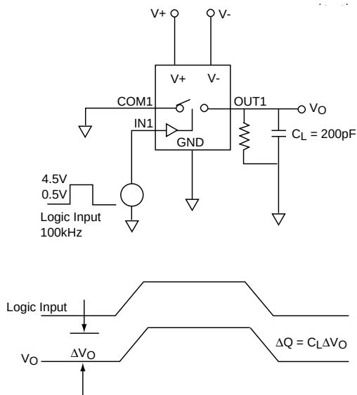
CHARGE INJECTION TEST CIRCUIT
