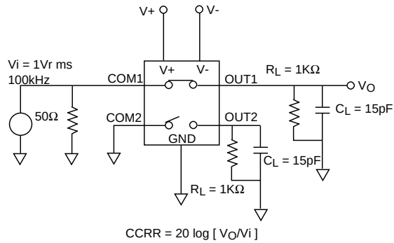
CROSSTALK TEST CIRCUIT
