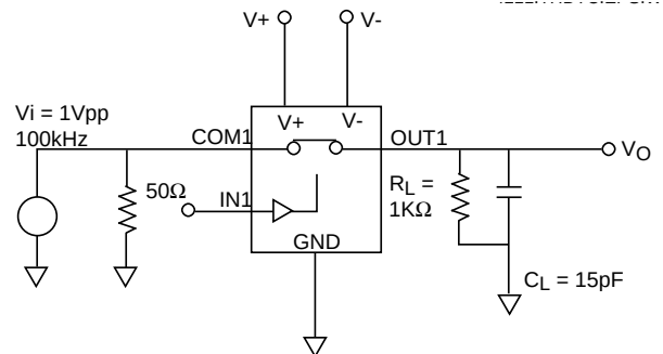
TOTAL HARMONIC DISTORTION TEST CIRCUIT
