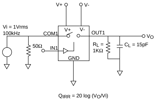
OFF ISOLATION TEST CIRCUIT
