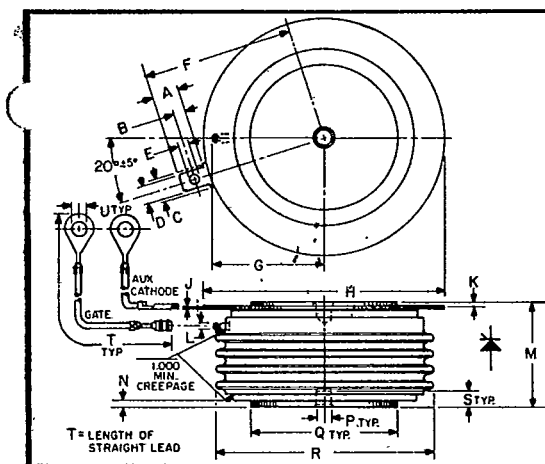
HP1 TABLE OF DIMENSIONS
