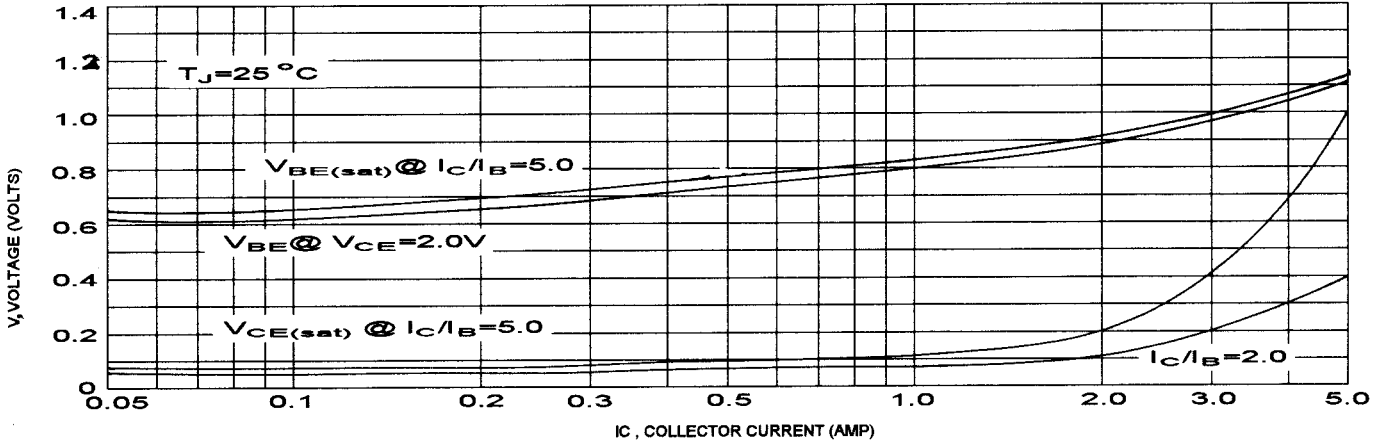
"ON" VOLTAGES
