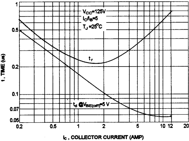
TURN-ON TIME
