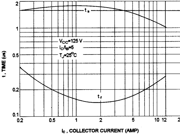
TURN-OFF TIME
