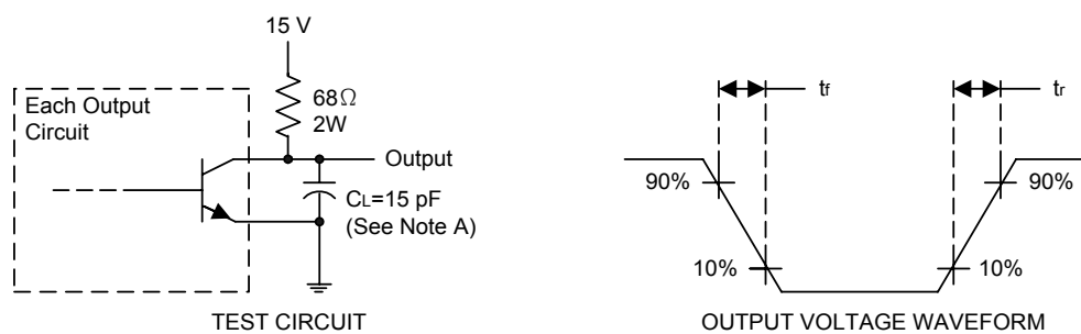
Figure 4. COMMON-EMITTER CONFIGURATION
