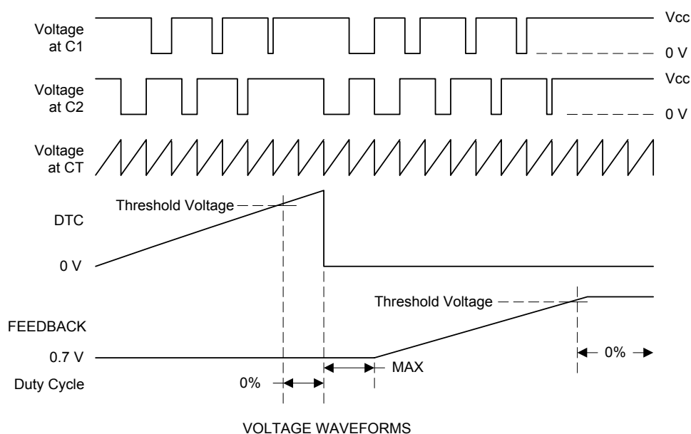
Figure 3. AMPLIFIER CHARACTERISTICS
