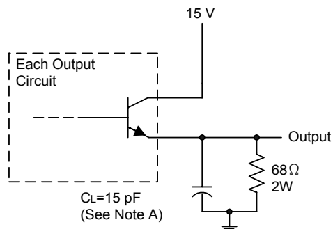
Figure 5. EMITTER-FOLLOWER CONFIGURATION
