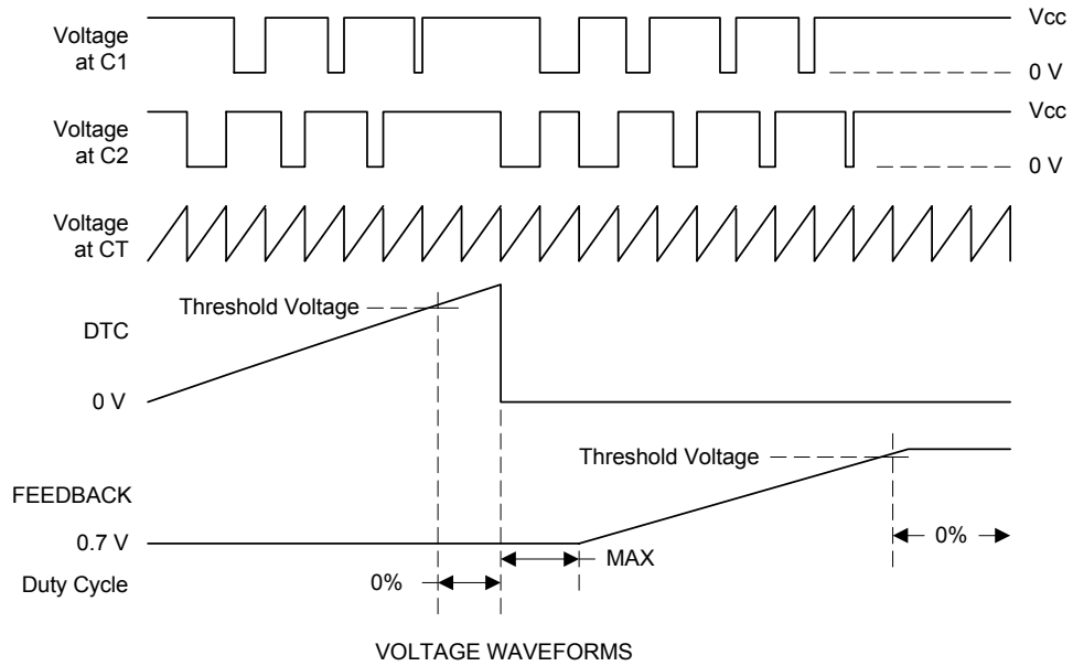
Figure 3. AMPLIFIER CHARACTERISTICS
