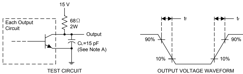
Figure 4. COMMON-EMITTER CONFIGURATION
