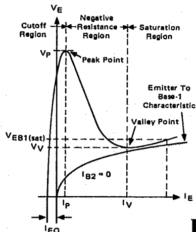
FIGURE 2 STATIC EMITTER CHARACTERISTIC CURVES
