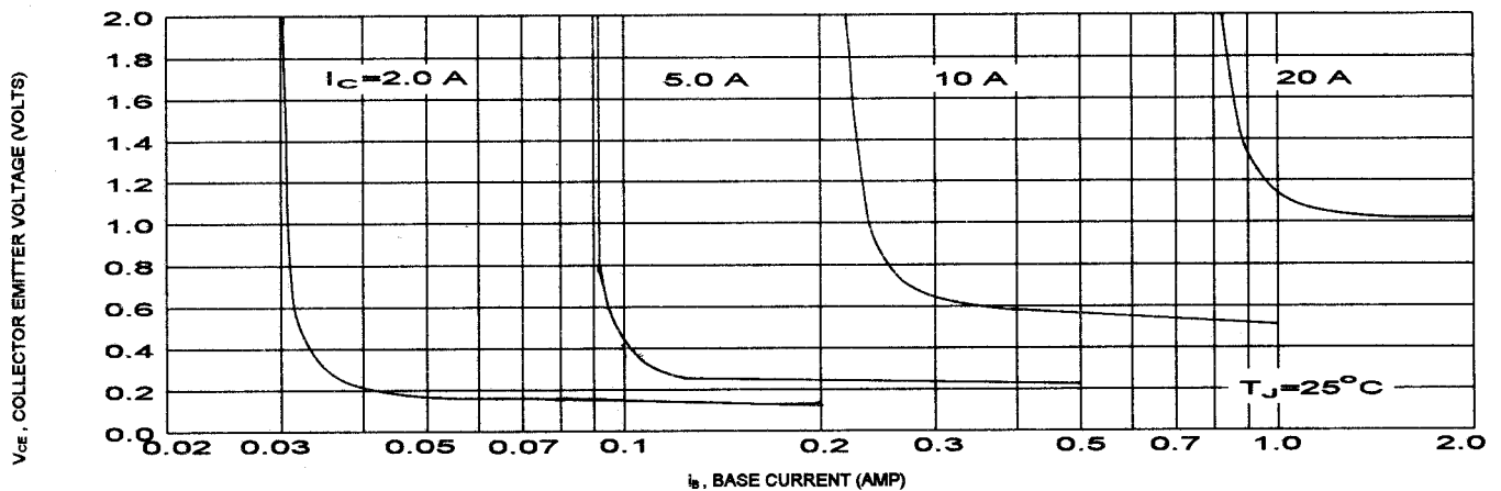
"ON" VOLTAGES
