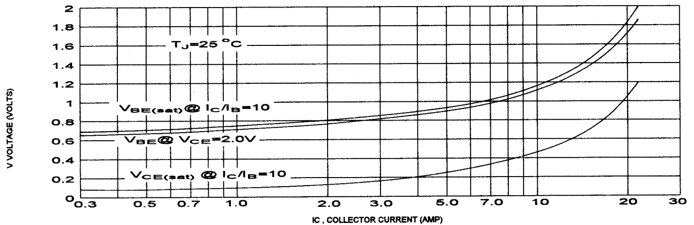
"ON" VOLTAGES
