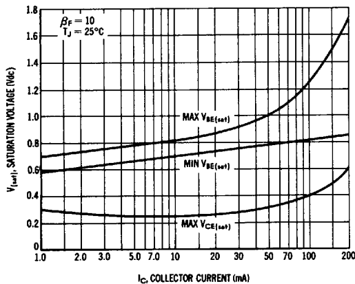
FIGURE 3 — LIMITS OF SATURATION VOLTAGES
